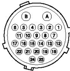
(Rear of connector VIEW)
